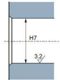
Mating Housing
